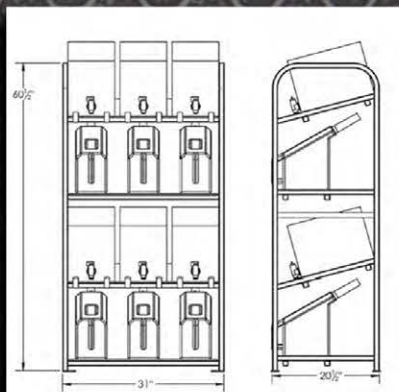
Rack System Part Number 880046
